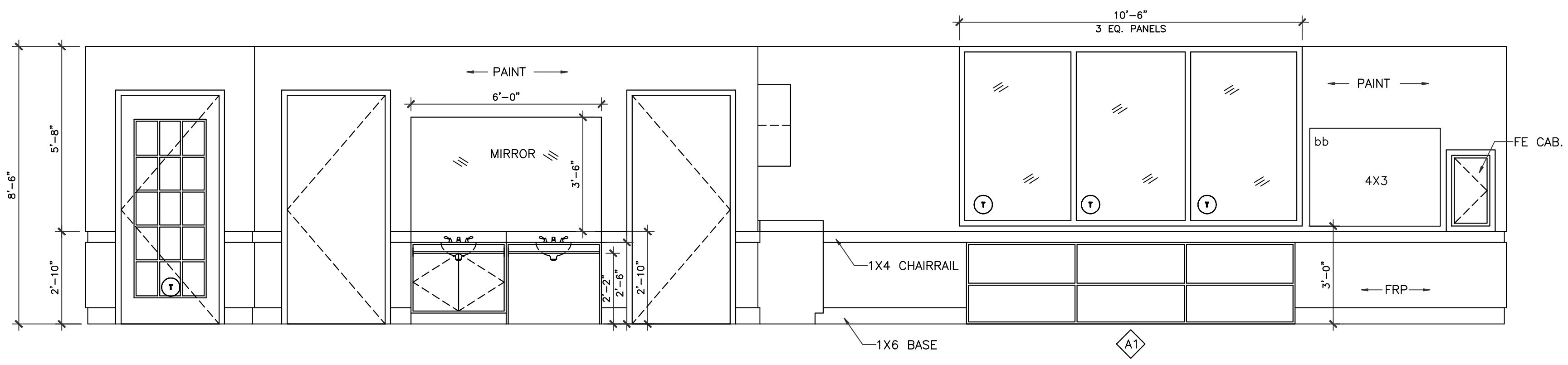
9 CLASSROOM ELEVATION 3/8" = 1'-0"
